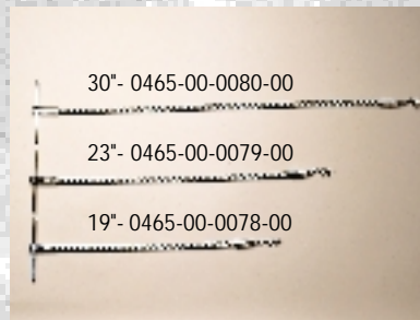
Flexible Shaft - Non-Removable Tip
