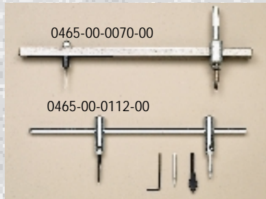
0465-00-0070-00 0465-00-0112-00 Gasket Cutter (2 styles) - (1" - 22" circle)
