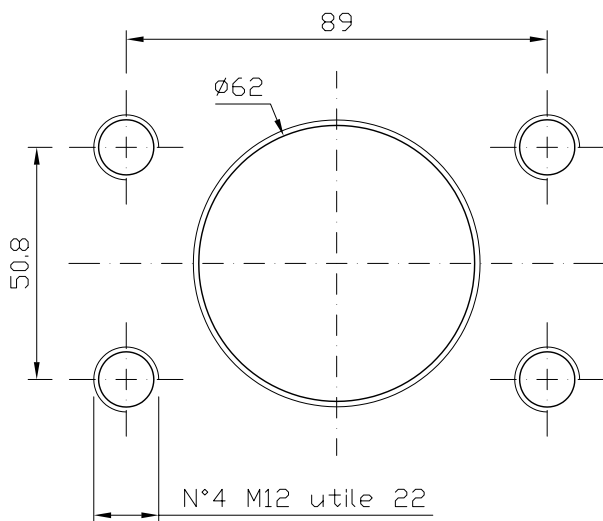
Inlet
