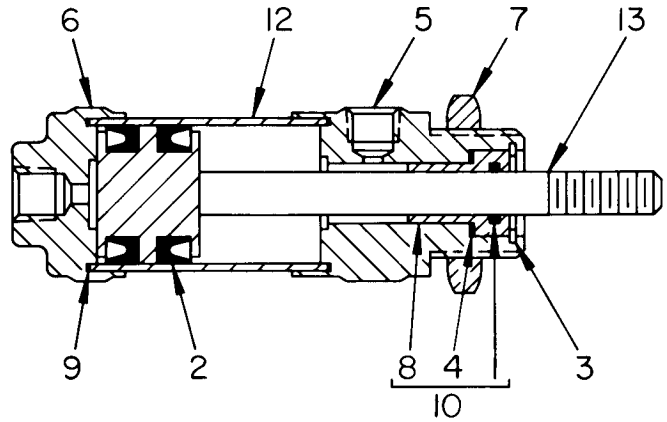
DOUBLE ACTING NECK MOUNTING
