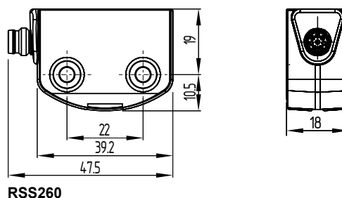
Dimensional drawing Safety sensor
