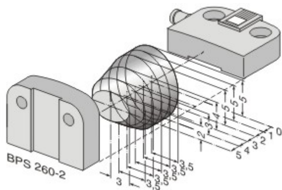
Dimensional drawing (basic component)
