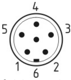
Contact arrangement
