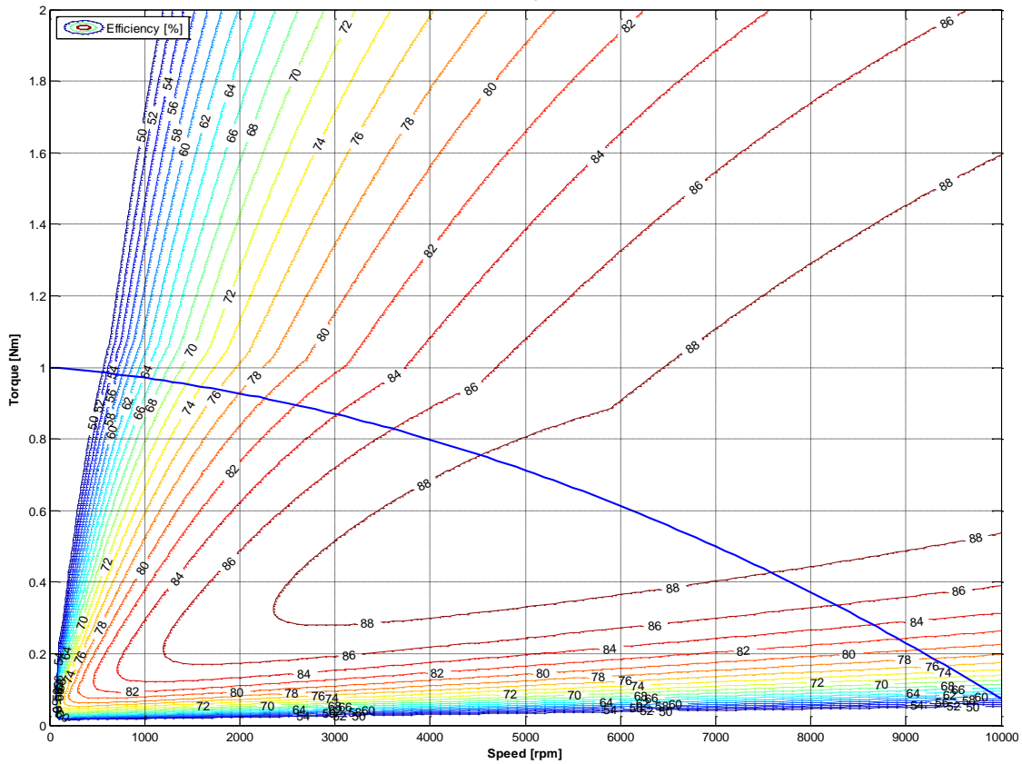
Constant efficiency curves of the motor NX310E
