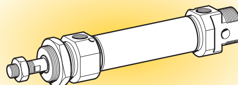
Double acting \varnothing 20 - \varnothing 25 , adjustable end-cushioning
