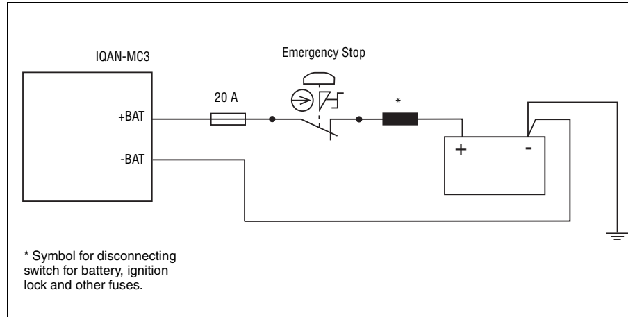
Connecting the emergency stop and voltage supply.
