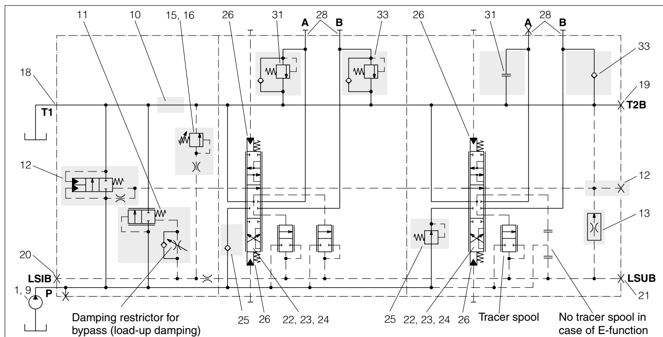
Diagram for basic functions shows HV08 in CFC version with two spool sections.
