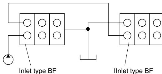
Series connection, CFC
