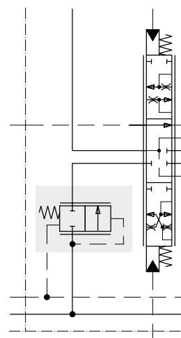
PR - Prioritizing valve in pressure gallery.
