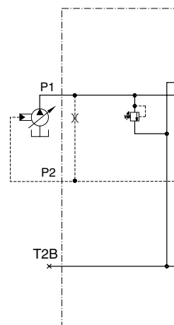
Standard inlet I with CUI-function and main pressure-relief function PS (F130CP).
