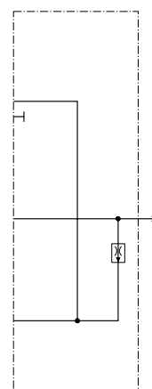
Free-flow gallery connected with tank through LD at item [33]. F130LS. only.
