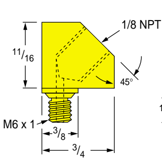
89 M6 to 1/8 (F) 45°
