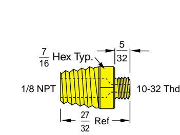
90 AN 1/8 to 10-32
