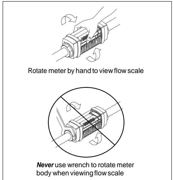
Figure 5. Rotating Meter
