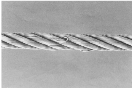
Wire protrusion
