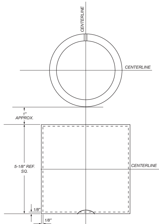
Large Press Base Dimensions Models 12, 19, 24, 38, & 58
