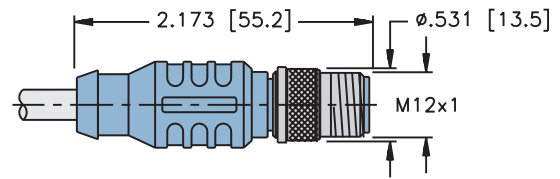
eurofast connector
