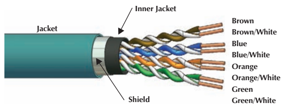
8-Wire Ethernet Cable
