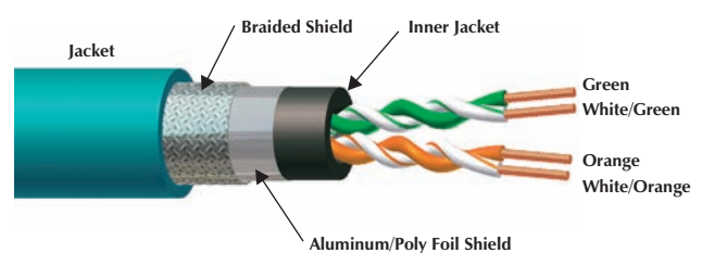
4-Wire Ethernet Cable
