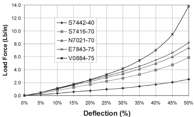
Chart 11 - Hollow-O (O.D. = .139", I.D. = .070")
