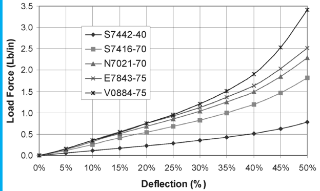
Chart 8 - Hollow-O (O.D. = .070", I.D. = .040")
