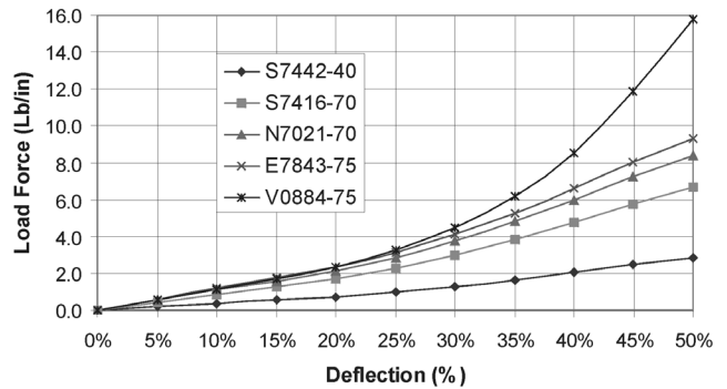
Chart 22 - Hollow-D (A = .312", B = .156", C = .156", D = .045")
