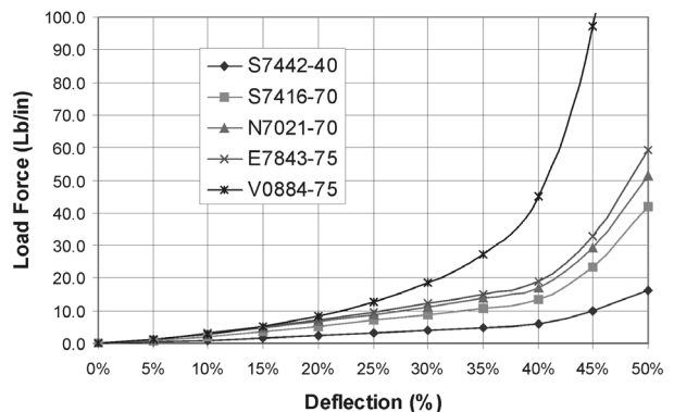
Chart 12 - Hollow-O (O.D. = .156", I.D. = .050")
