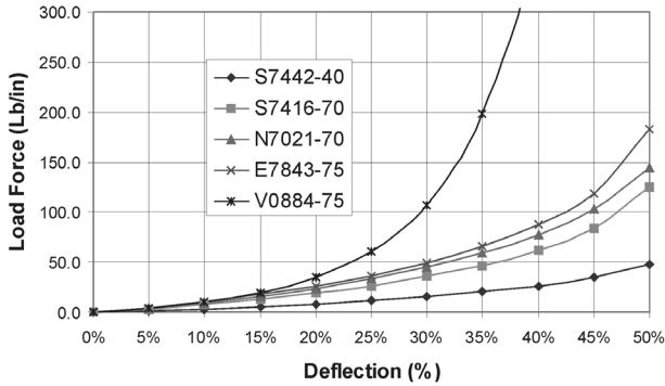
Chart 19 - Square (Edge = .099")
