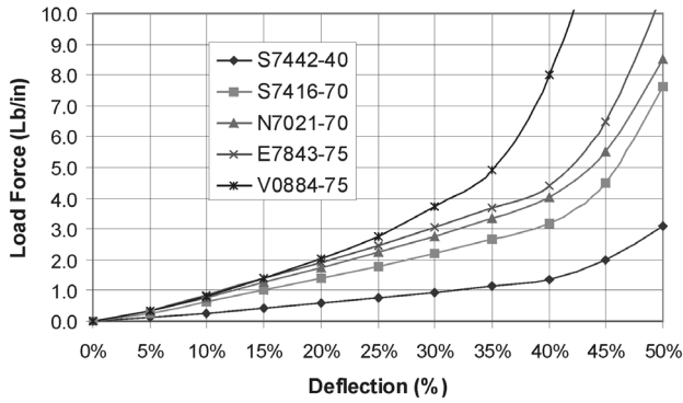
Chart 7 - Hollow-O (O.D. = .070", I.D. = .030")
