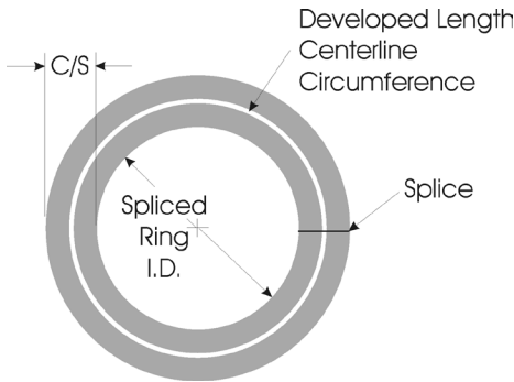
Figure 1 - Developed Length
