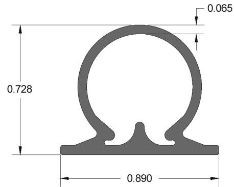
Figure 7 - Simple Drawing of Omega Profile
