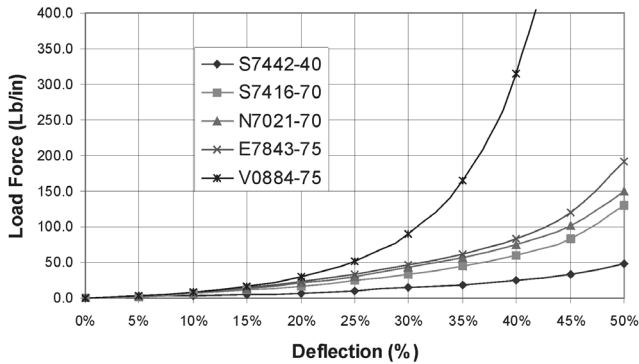
Chart 21 - Solid-D (H = .156", W = .156", R = .078")
