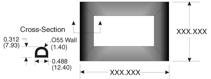
Figure 2 - Typical TechSeal Picture Frame Gasket
