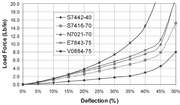
Chart 9 - Hollow-O (O.D. = .103", I.D. = .040")
