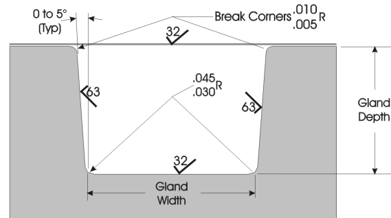
Figure 4 - Typical Gland Surface Finish
