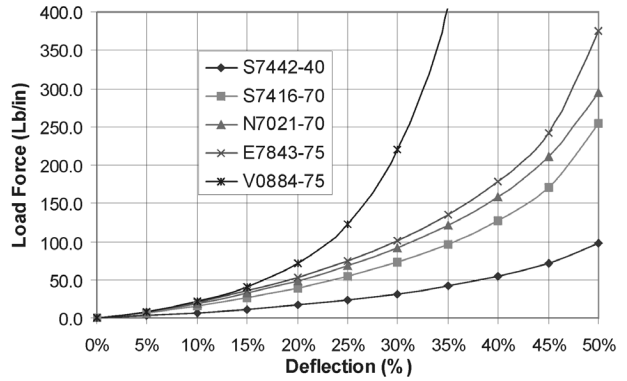
Chart 20 - Square (Edge = .203")
