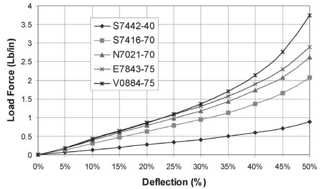
Chart 10 - Hollow-O (O.D. = .103", I.D. = .062")
