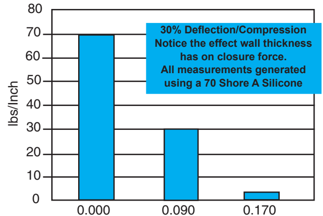
Figure 6 - Effect of geometry on closure force
