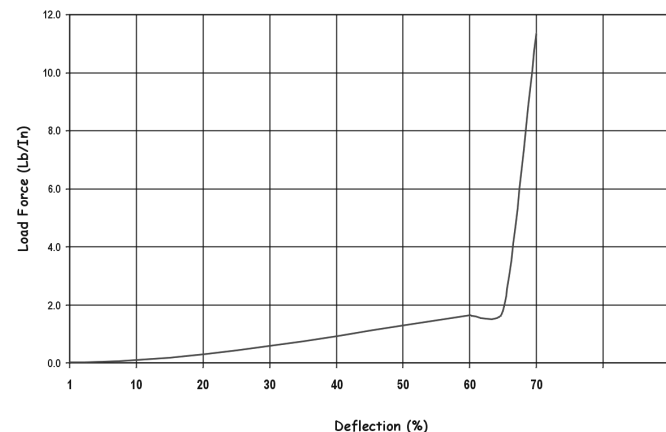
Figure 8 - FEA Generated Deflection Curve
