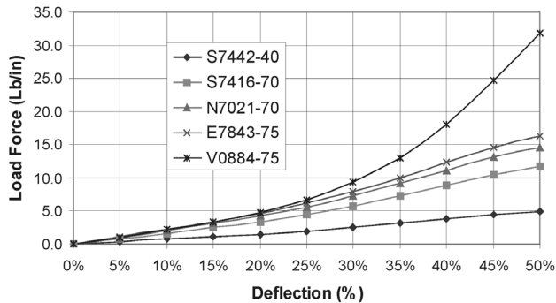
Chart 23 - Hollow-D (A = .488", B = .068", C = .244", D = .055")
