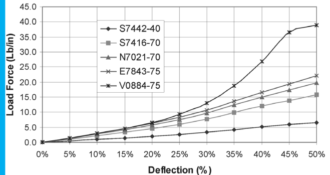
Chart 24 - Hollow-D (A = .312", B = .156", C = .156", D = .062")
