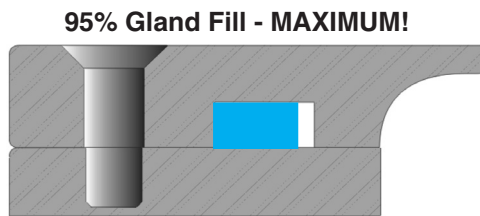
Figure 3 - Maximum Gland Fill Percentage
