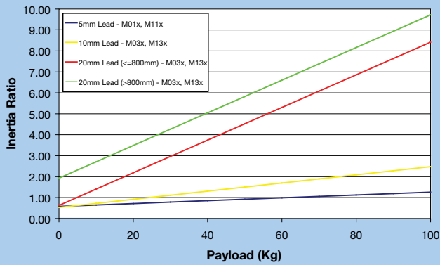
HD125 Inertia Ratios
