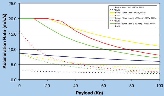
HD125 Acceleration Rates
