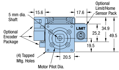
Enlarged End View (with Encoder and Limit/Home Sensor Pack Option)
