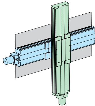
Figure 2 Two Axis (X-Z) Vertical Mounting
