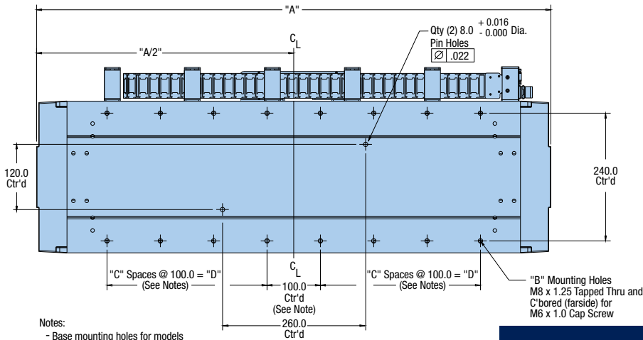
Bottom View
