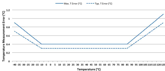
Temperature Accuracy
