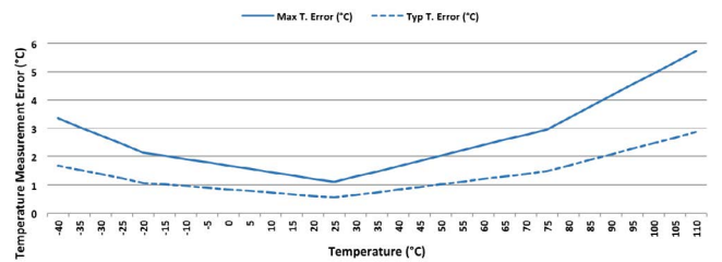
Temperature Accuracy
