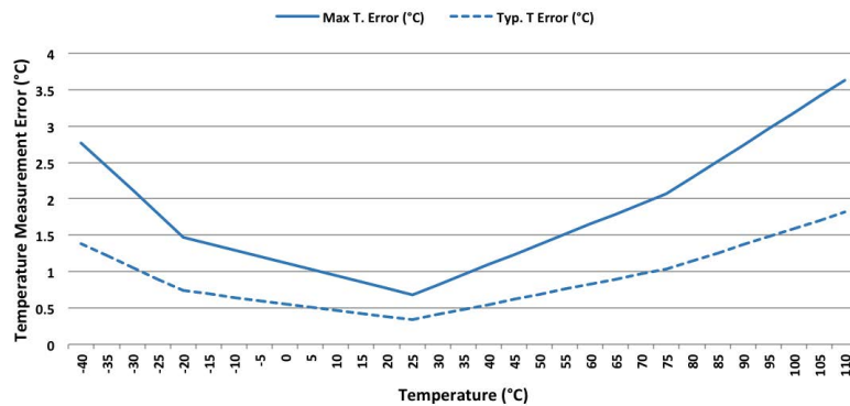
Temperature Accuracy
