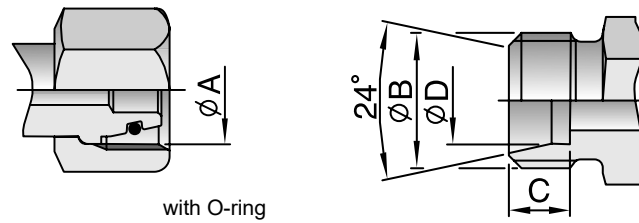
with O-ring
