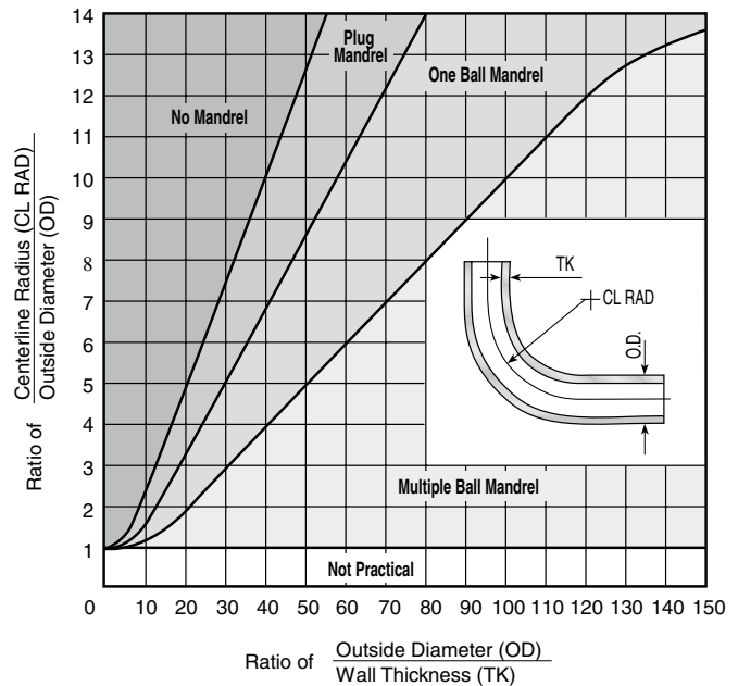
Fig. S57 — Mandrel bending requirements chart
