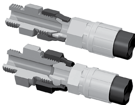
Fig. H1 – JIS T4 and P4 Interfaces
