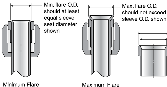
Fig. S29 — Comparing flare O.D. with sleeve seat and O.D.
