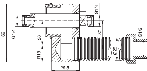
Outlet connection parallel P1V-6/388378A
