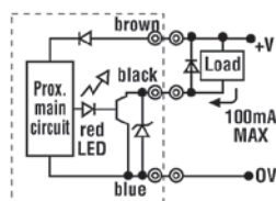
250-3 NPN NPN-type Proximity Switch
