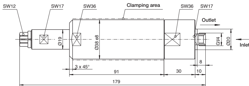
Outlet connection parallel P1V-6/388378A
