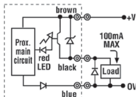
250-3 PNP PNP-type Proximity Switch
