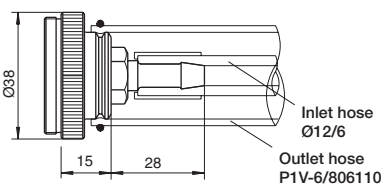
Outlet connection straight P1V-6/313179A
