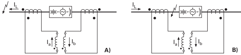
Schematic Circuit Diagrams (Single-Phase Version): A) Fault Outside the Protection Area B) Fault Inside the Protection Area
